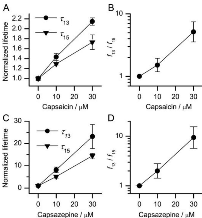
Fig. 4. Effects of capsaicin or capsazepine on channels formed by 15 amino acid monomers ([Ala 1 ]gA (15 amino acids) and 13 amino acids [des-Val 1 -Gly 2 ]gA - ). A, capsaicin-induced changes in channel lifetimes ( \tau_{15} and \tau_{13} , respectively). B, capsaicin-induced changes in the ratio of appearance rates of [des-Val 1 -Gly 2 ]gA - and [Ala 1 ]gA and channels ( f_{13}/f_{15} ). C, capsazepine-induced changes in \tau_{15} and \tau_{13} . D, capsazepine-induced changes in ( f_{13}/f_{15} ).
